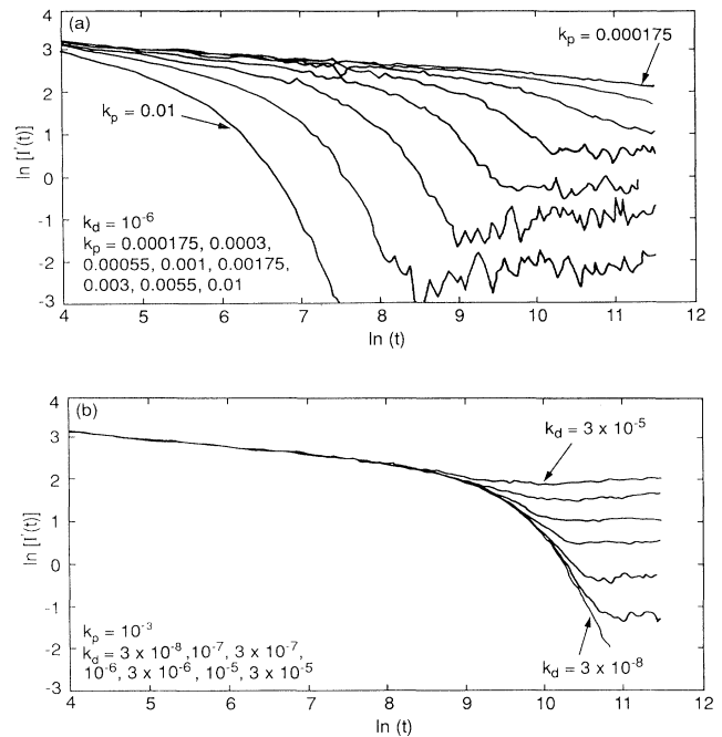
FIG. 9. Mean current profiles I'(t) obtained from the single-pit model. Part (a) shows results obtained with a constant depassivation rate constant ( k_d = 10^{-6} ) and eight different passivation rate constants. Part (b) shows results obtained with a constant passivation rate constant ( k_p = 10^{-3} ) and seven depassivation rate constants. Here I' is 100I(t) .
